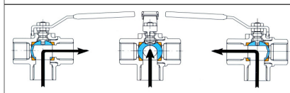
L – Port Configuration
