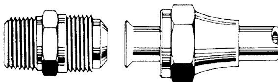
THREADS USED ON THE MALE FLARE END
